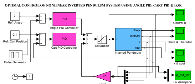
Figure 4. Angle PID, Cart PID & LQR Control of Nonlinear Inverted Pendulum System.
