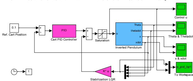
OPTIMAL CONTROL OF NONLINEAR INVERTED PENDULUM SYSTEM USING CART PID & LQR
