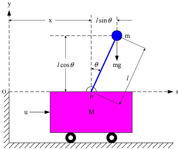
Inverted Pendulum - Cart System
