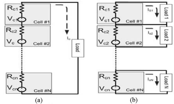
Fig. 5. Modular fuel cell simplified equivalent circuit.
