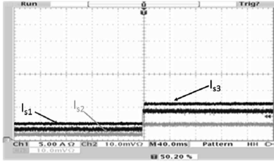
Fig. 12. Modular fuel cell section currents during a load transient.
