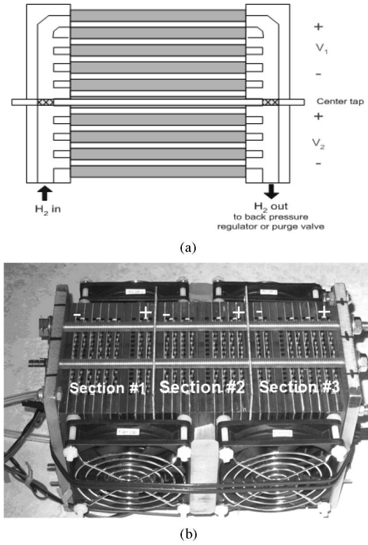
Fig. 6. (a) Schematic drawing of the modular fuel cell stack. (b) Prototype of the 12-V, 150-W, 24-cell modular fuel cell stack.
