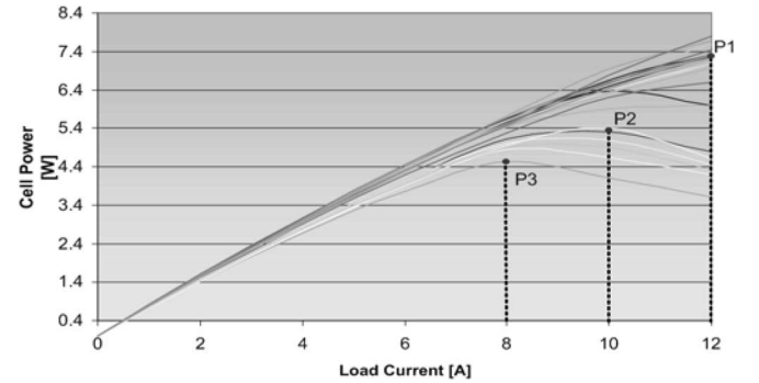
Fig. 4. Individual cell P – I .
