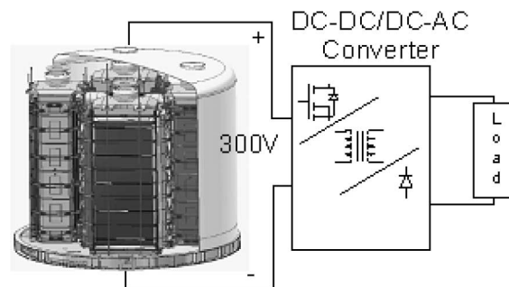
Fig. 1. Utility scale fuel cell stack and dc–dc/dc–ac converter.
