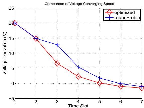
Fig. 5: Comparison of voltage at sensor 1.
