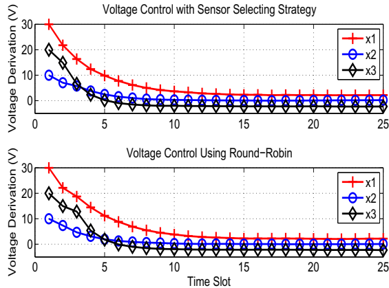
Fig. 3: Voltage evolution with time.
