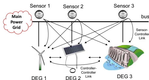
Fig. 1: An illustration of the voltage control in micro grid.
