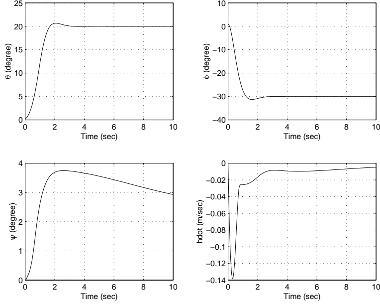
Figure 2: Outputs of helicopter state without noise or Kalman filtering
