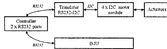
Fig. 4. OS4 test-bench block diagram
