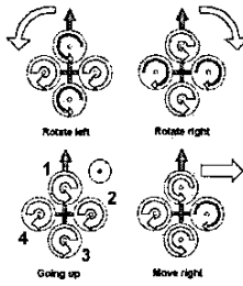
Fig. 1. Quadrotor concept rotational motion description, the arrow width is proportional to propeller rotational speed.
