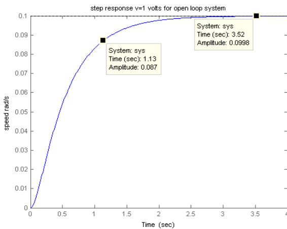
Fig(3): response open loop
