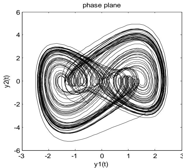
Figure 3: Phase portrait of \Phi^6 -Van Der Pol oscillator
