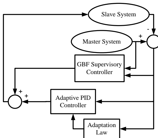
Figure 1: Schematic diagram of a synchronization mechanism
