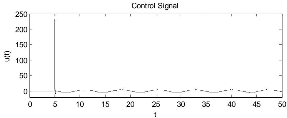
Figure 9: The control signal with GBFC
