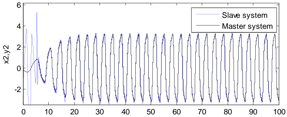
Figure 4: Time response of controlled chaotic \Phi_6 -van der pol synchronization system
