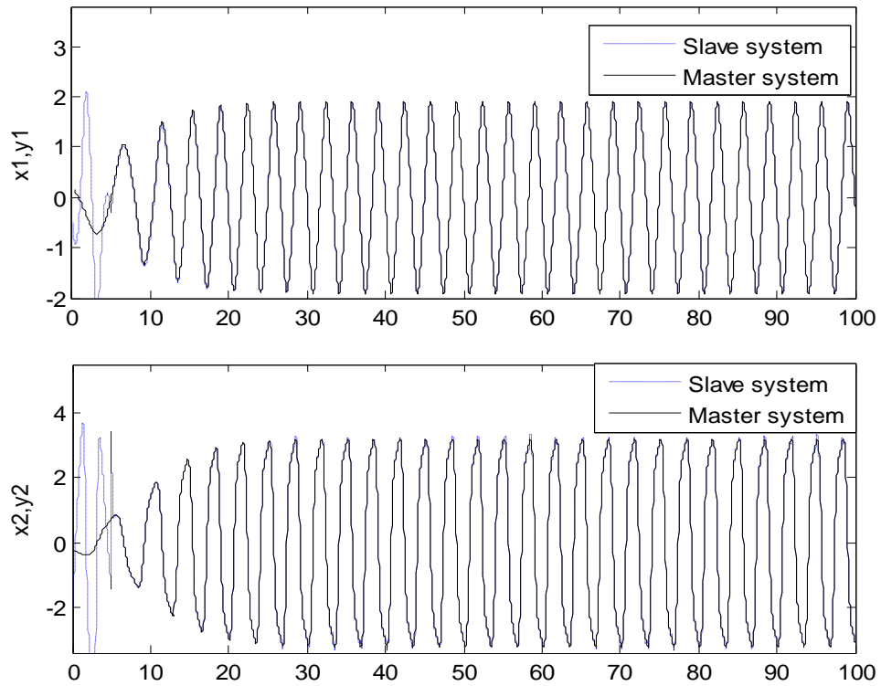
Figure 7: Time response of GBFC synchronization \Phi_6 -van der pol
