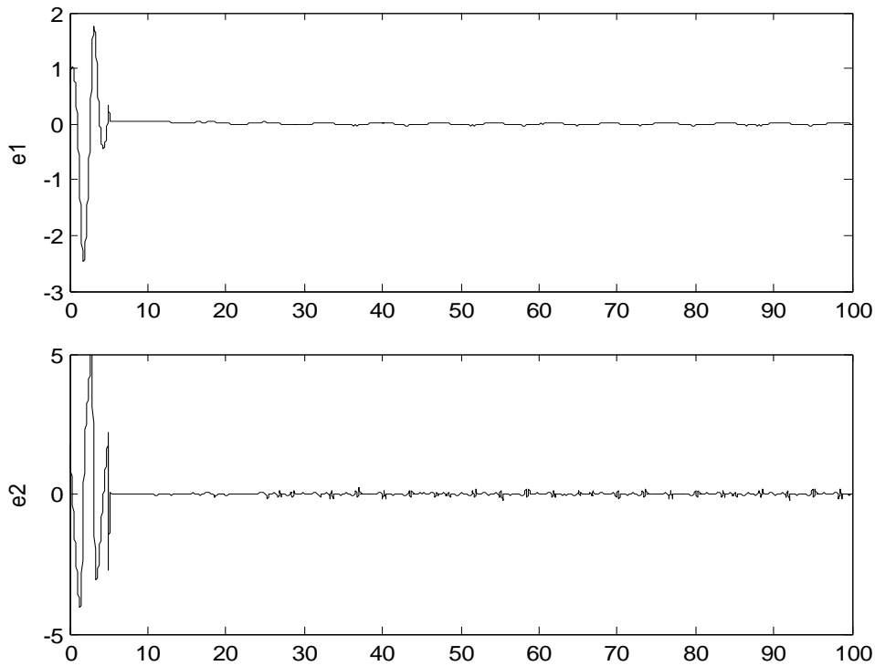
Figure10: The synchronization error of Master and Slave \Phi_6 -van der pol
