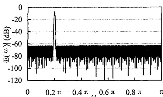
Fig. 1 The weighted error of the filter in example 1
