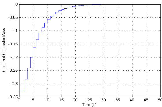
Fig .2-a the normalized mass in combustor chamber x_1(k)
