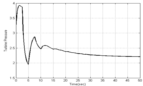
Fig.4-b turbine total inlet pressure z_2(t)
