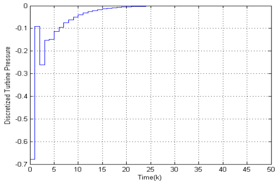
Fig .2-b the normalized inlet turbine pressure x_2(k)
