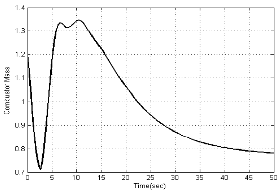
Fig .4-a mass in combustion chamber z_1(t)
