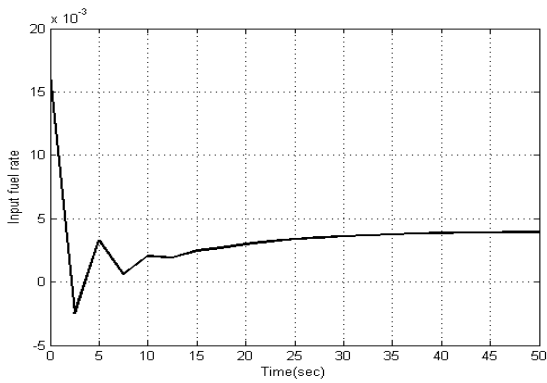
Fig. 4-d mass fuel rate w = \frac{\dot{m}_{fuel}}{\dot{m}_r} \cong \tilde{w}(k) = F^T z(t) + v_o .
