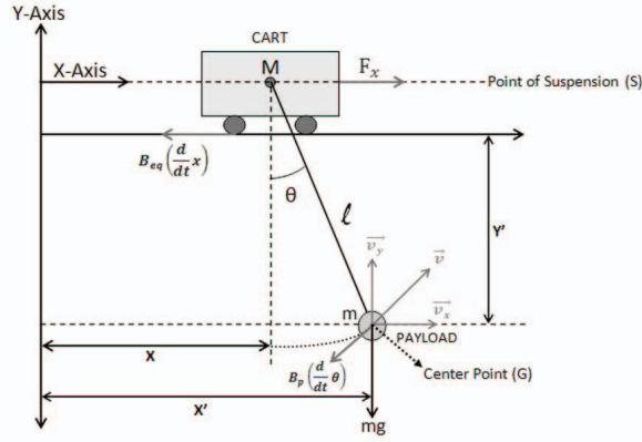
FIG.1: SPGC Model
