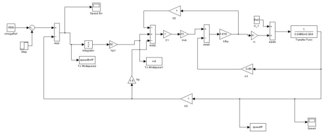
Fig 9. I-P controller
