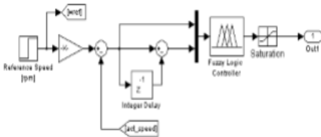
Fig 10. Block Diagram of FLC
