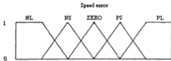
Fig 4. Set of linguistic variables
