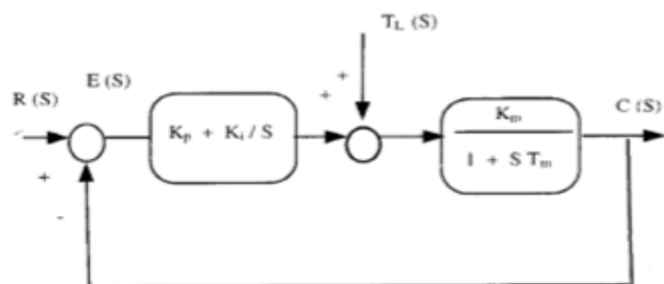
Fig 1. Block diagram with P-I controller
