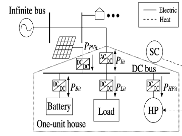
Fig. 2. DC smart-house model.
