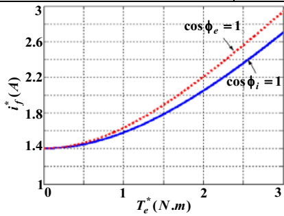
Figure 5. The relation between the rotor current and torque
