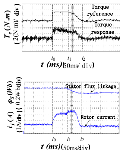
Figure 14. Field weakening operation from 750\text{r.min}^{-1} to 2000\text{r.min}^{-1}
