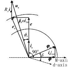
Figure 3. The vector diagram with unity inner power factor
