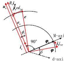
Figure 4. The vector diagram with unity outer power factor
