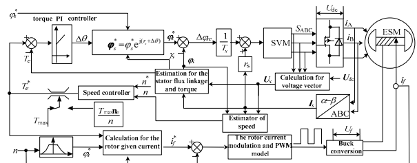
Figure 10. System diagram of the ESM SVM-DTC
