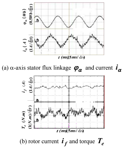
Figure 16. the steady state experimental waveforms at the 2000r.min -1 with 1.5N.m load
