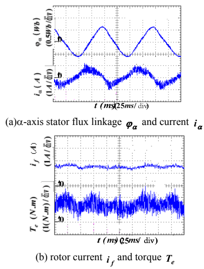
Figure 15. the steady state experimental waveforms at the 300r.min -1 with 1.5N.m load
