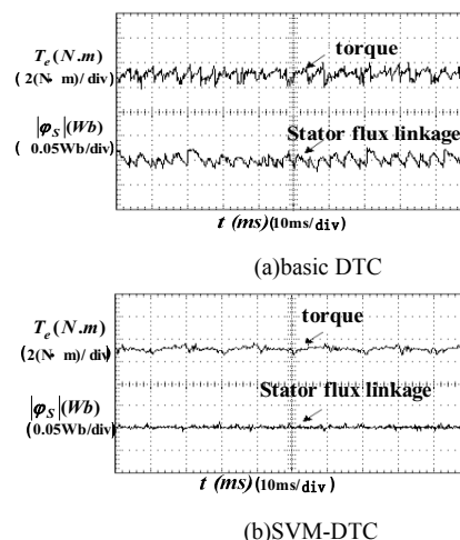
Figure 12. The experimental waveforms of torque and stator flux linkage at 1500\text{r.min}^{-1} with no load
