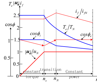
Figure 2. The optimum rotor current control strategy for vector controlled ESMs
