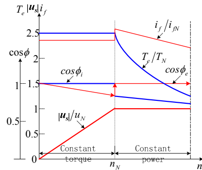
Figure 9. The presented optimum rotor current control strategy for DTC ESMs
