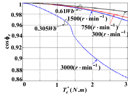
Figure 8. The relation between the outer power factor and torque
