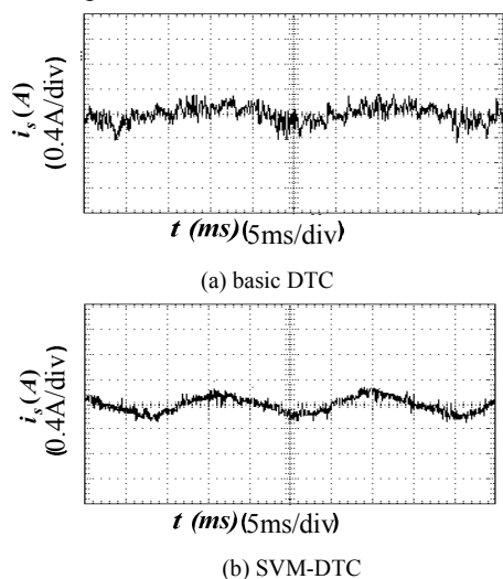
Figure 11. The experimental waveforms of phase current at 1500\text{r.min}^{-1} with no load
