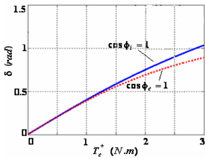
Figure 6. The relation between the load angle and torque
