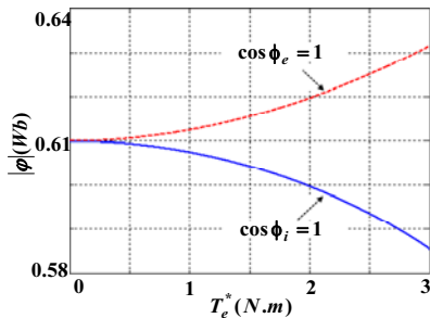
Figure 7. The relation between the air gap flux linkage modulus and the torque
