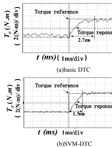
Figure 13. The experimental waveforms of torque step response
