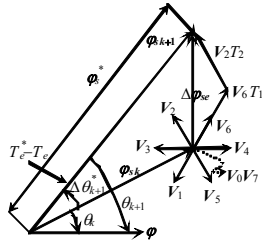
Figure 1. The control principle for torque and stator flux linkage
