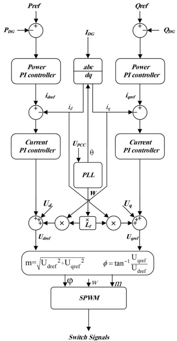
Fig. 2 DG controller scheme
