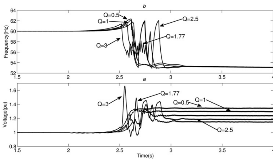
Fig. 11 Islanding detection for different values of quality factors
