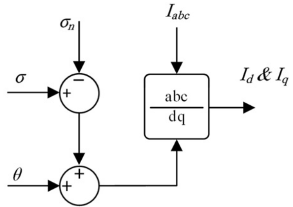
Fig. 3 Additional block of the proposed method
