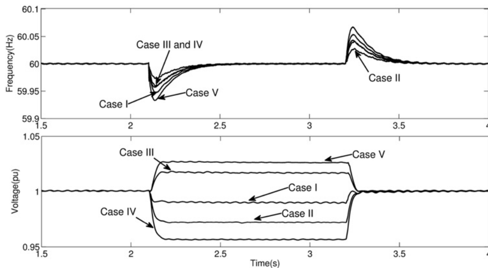
Fig. 7 Frequency and voltage variations during load switching
