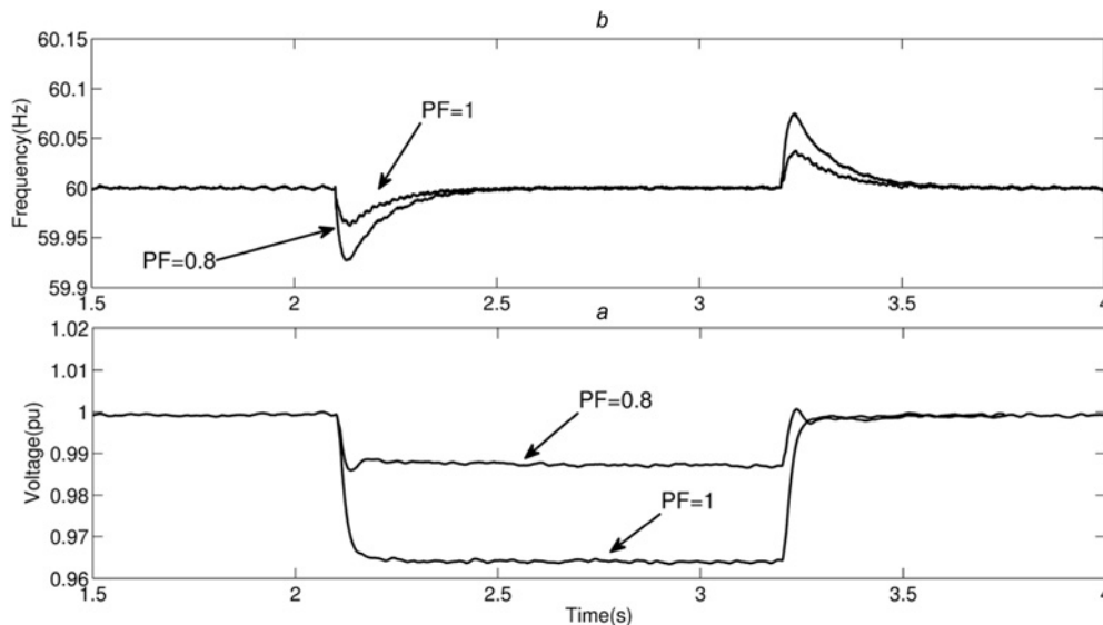
Fig. 14 Frequency and voltage variations during load switching for multiple DGs
