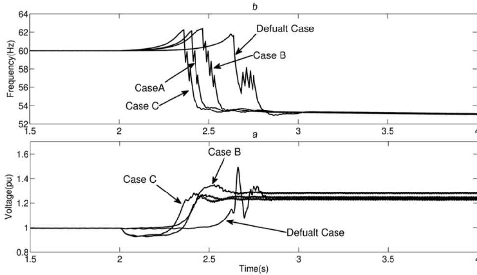
Fig. 12 Frequency and voltage variations for unbalanced load conditions
