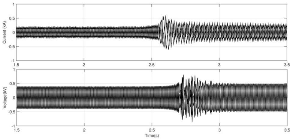
Fig. 5 Waveform of voltage and current
