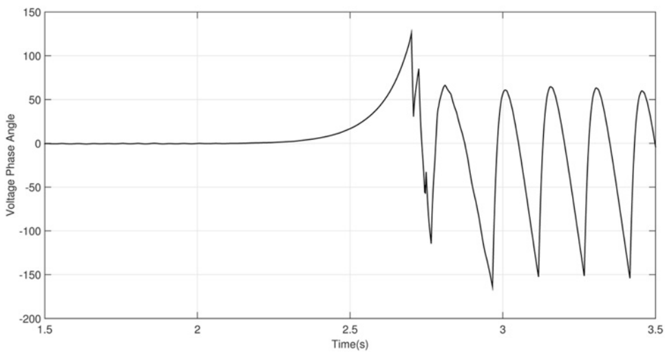
Fig. 6 Amplitude of error between the instantaneous VPA ( \sigma ) and the nominal VPA of DG ( \sigma_n )
