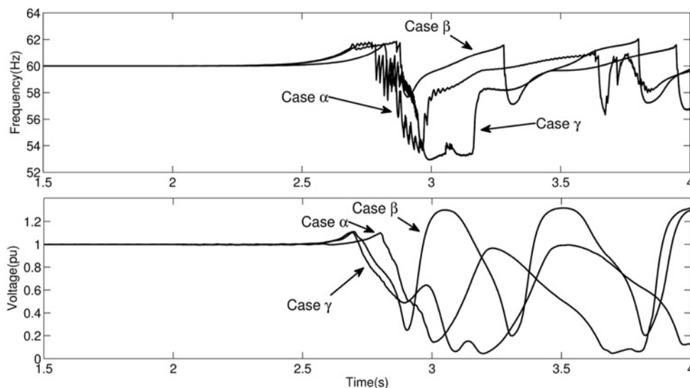
Fig. 13 Frequency and voltage variations after islanding occurrence for multiple DGs with proposed method
