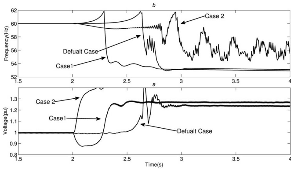
Fig. 9 Frequency and voltage variations for cases 1, 2 and default case
