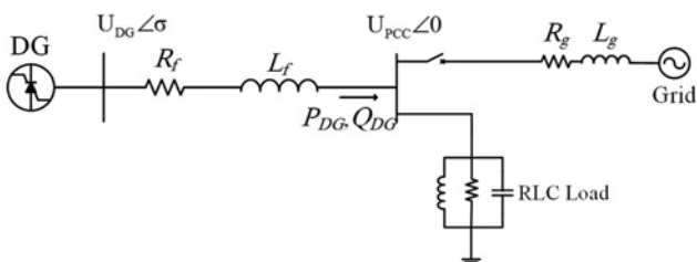
Fig. 1 System under study
