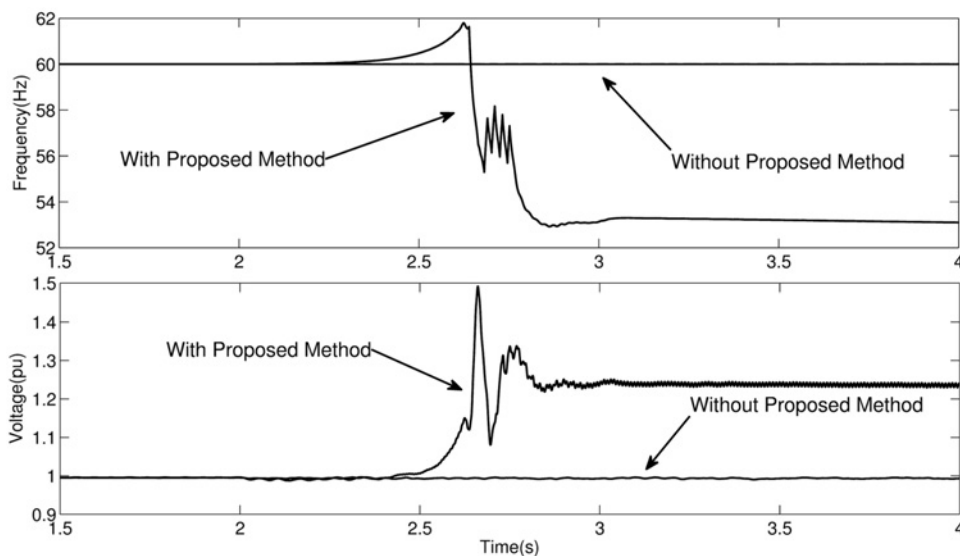
Fig. 4 Islanding detection with proposed method for default cases
