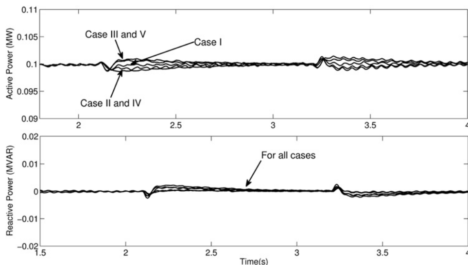
Fig. 8 Active and reactive power variations during load switching
