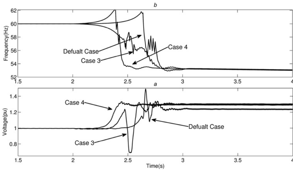
Fig. 10 Frequency and voltage variations of unbalanced conditions of reactive power
