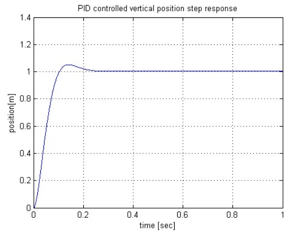
Fig. 6. PID Vertical position step response.
