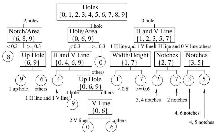
FIGURE 3. The decision tree for our DTC
