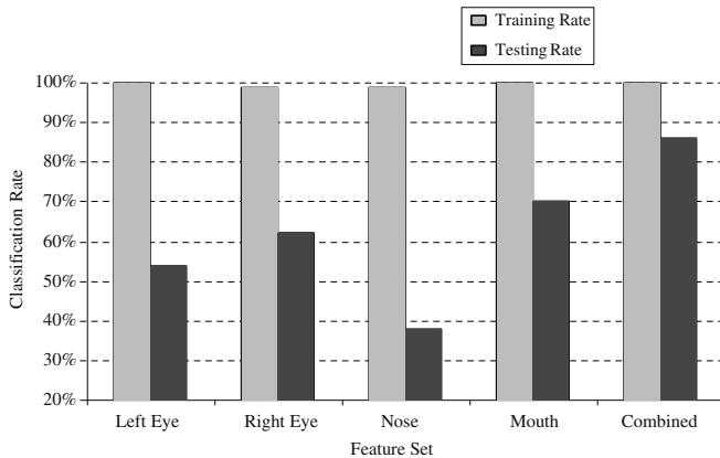
Fig. 5.1. Classification rate comparison between different feature sets.
