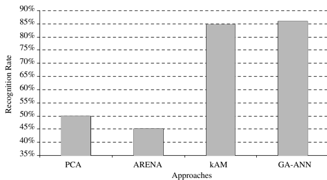
Fig. 5.2. Comparison with other approaches. (3 images per class for training set).
