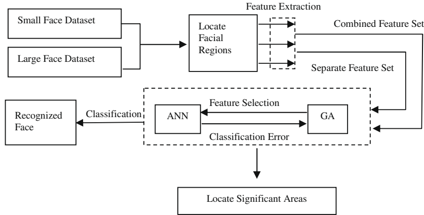
Fig. 2.1. Block diagram of the proposed technique.
