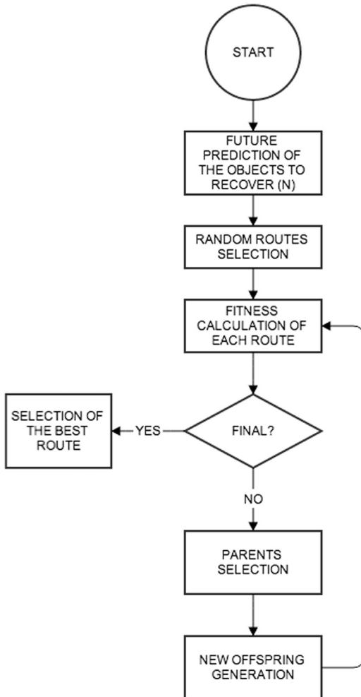
Fig. 3. GATP block diagram.
