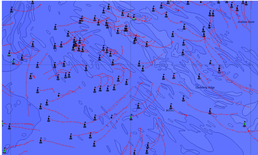
Fig. 1. FADs drifting in the Indian Ocean. (For interpretation of the references to color in this figure caption, the reader is referred to the web version of this article.)
