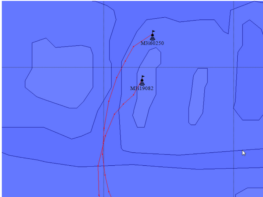
Fig. 2. Two FADs drifting in the ocean. (For interpretation of the references to color in this figure caption, the reader is referred to the web version of this article.)
