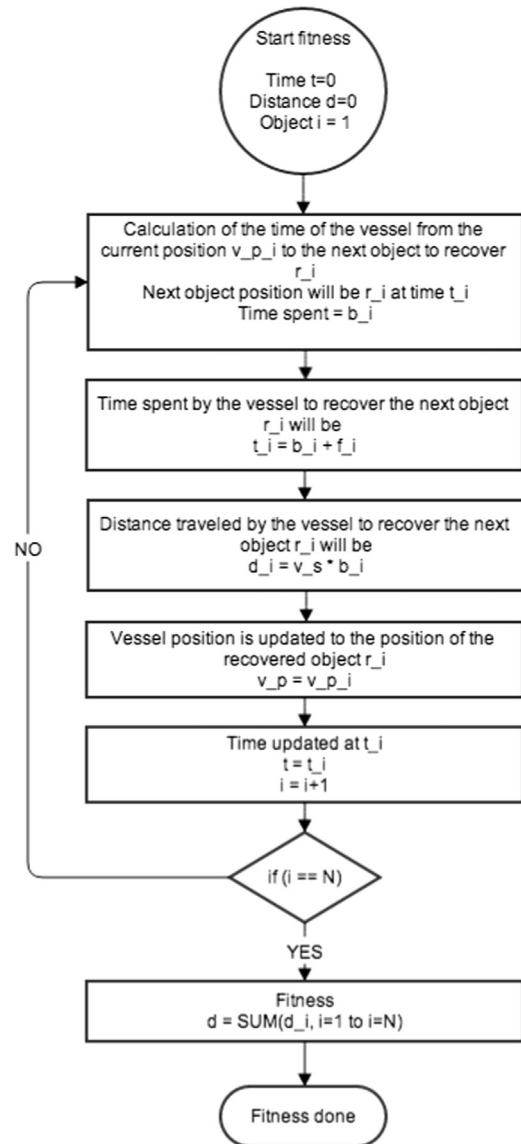
Fig. 4. GATP fitness calculation.
