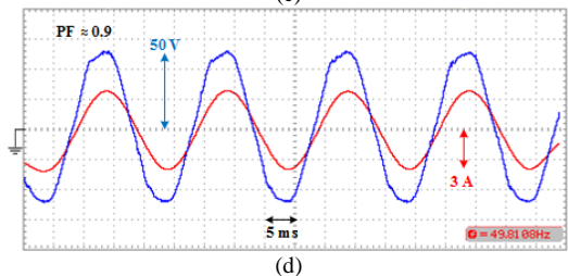
Fig. 12. Simulation and Experimental results for AC-DC converter in G2V mode: a) simulation result for V_s and I_s with PF=1; b) simulation result for V_s and I_s with PF=0.9; c) experimental results for with PF=1; d) experimental results for PF=0.9
