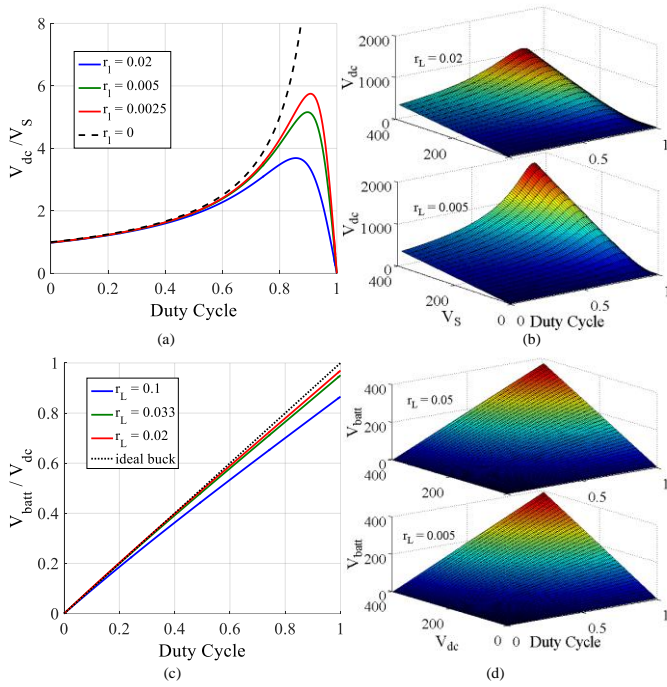
Fig. 3. H-bridge converter: a) V_{dc}/V_s ratio; b) Variation of V_{dc} vs. V_s and D ; DC-DC converter: c) V_{batt}/V_{dc} ratio; d) Variation of V_{batt} vs. V_{dc} and D
