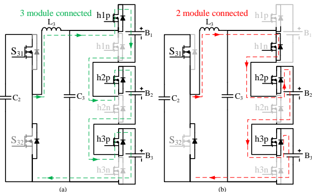
Fig. 4. Current path during the G2V mode: a) 3 modules connected; b) 2 modules connected
