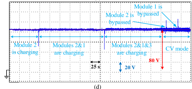
Fig. 13. Simulation and experimental results for DC link voltage during G2V mode: simulation results during a) the start-up, b) the CE procedure; experimental results during c) the start-up, d) the CE procedure
