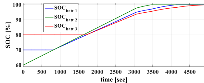
Fig. 11. SOC of the battery modules during the G2V mode
