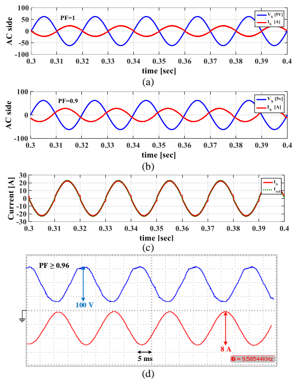
Fig. 17. Simulation and experimental results for AC-DC converter in the V2G mode: a) simulation result for V_S and I_S with PF=1; b) simulation result for V_S and I_S with PF=0.9; c) simulation result for I_S and I_{ref} ; d) experimental results for V_S and I_S with unity power factor
