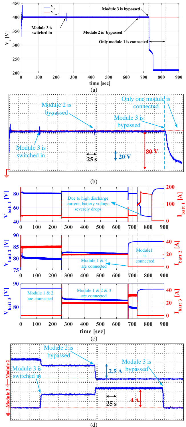
Fig. 16. DC side during V2G: a) simulation result of DC link voltage during CE; b) experimental result of DC link voltage during CE; c) simulation result for battery pack voltage and current; d) experimental results for the battery pack currents.
