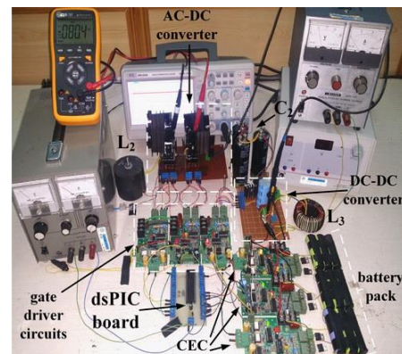
Fig. 10. The implemented system in the laboratory
