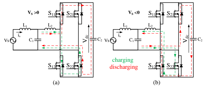
Fig. 2. Current path during G2V operation: a) V_s > 0 ; b) V_s < 0
