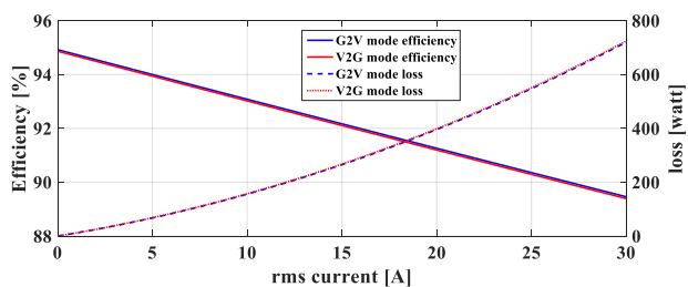
Fig. 18. Total efficiency and power loss during G2V and V2G operation
