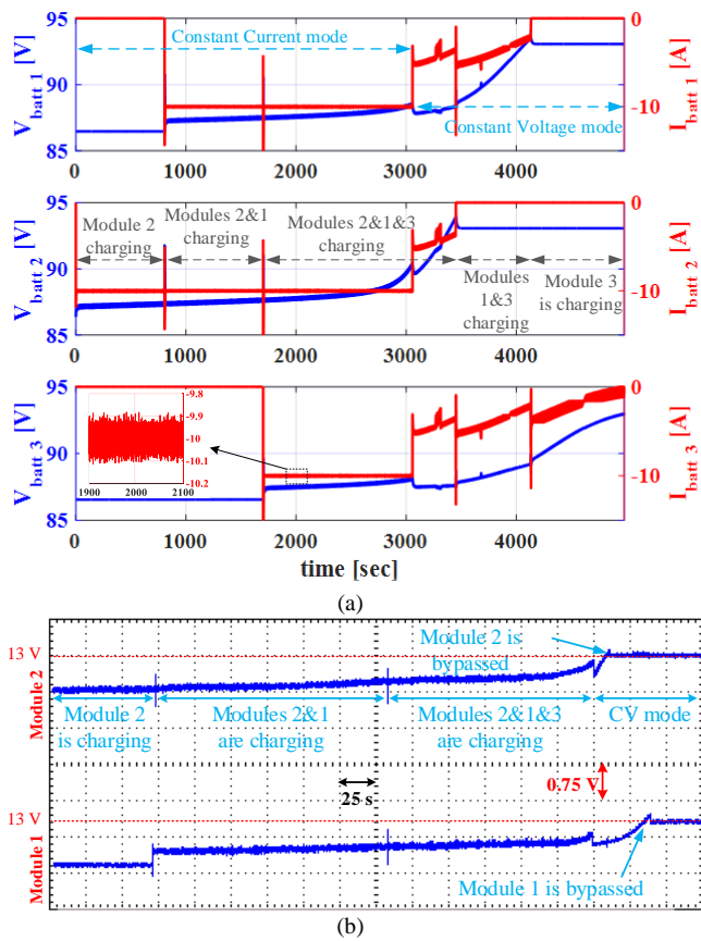
Fig. 14. G2V operation: a) simulation results for Battery modules Voltage and current; b) experimental battery voltage for module 1 and 2
