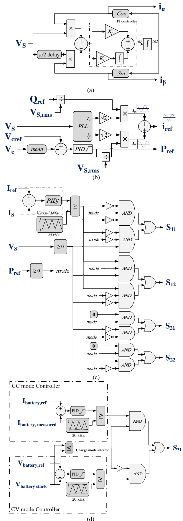
Fig. 6. AC-DC converter Controller: a) single-phase PLL; b) reference current control diagram in G2V mode; c) Current loop and switching control diagram; d) Control block diagram of the buck converter.
