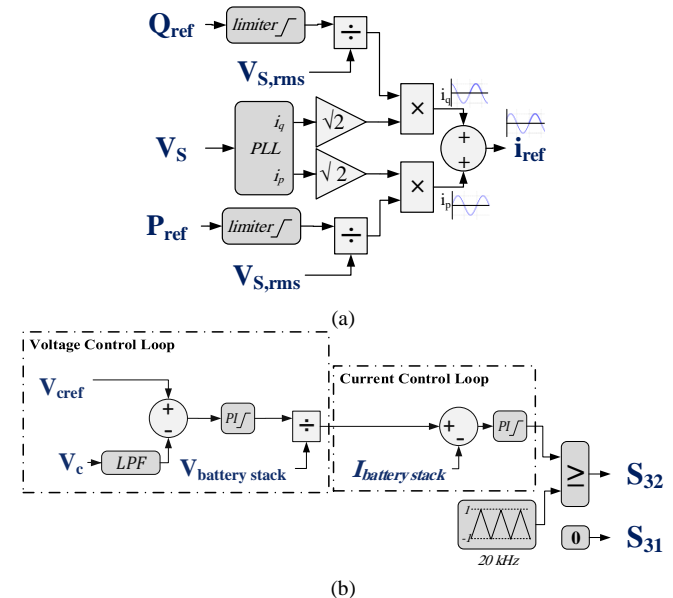
Fig. 8. V2G mode: a) Schematic of the reference current control in the V2G mode; b) Schematic of the step-up converter control during V2G mode.
