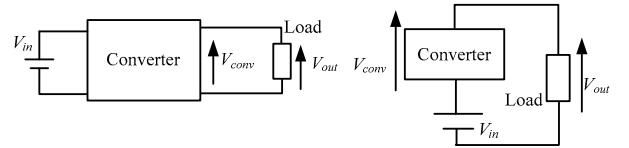
(a) Conventional topology.
